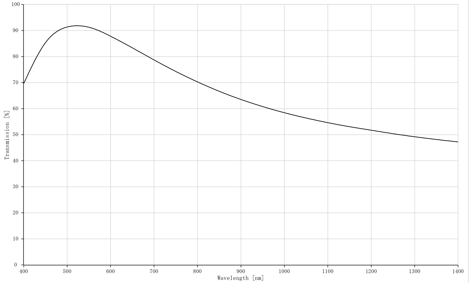
LM8JC5MC-WP Transmission
