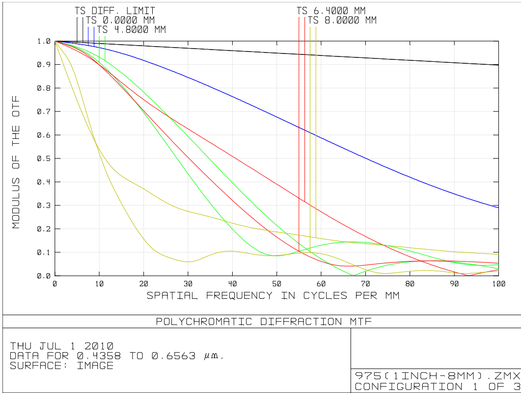
MTF (Object \infty )/ F1.4
