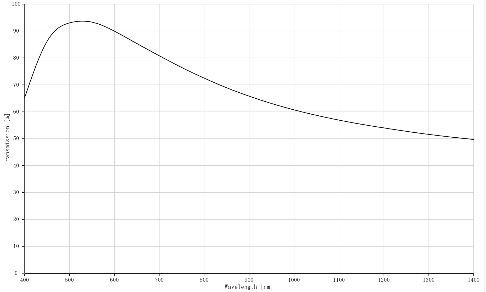
LM16JC5MC-WP Transmission
