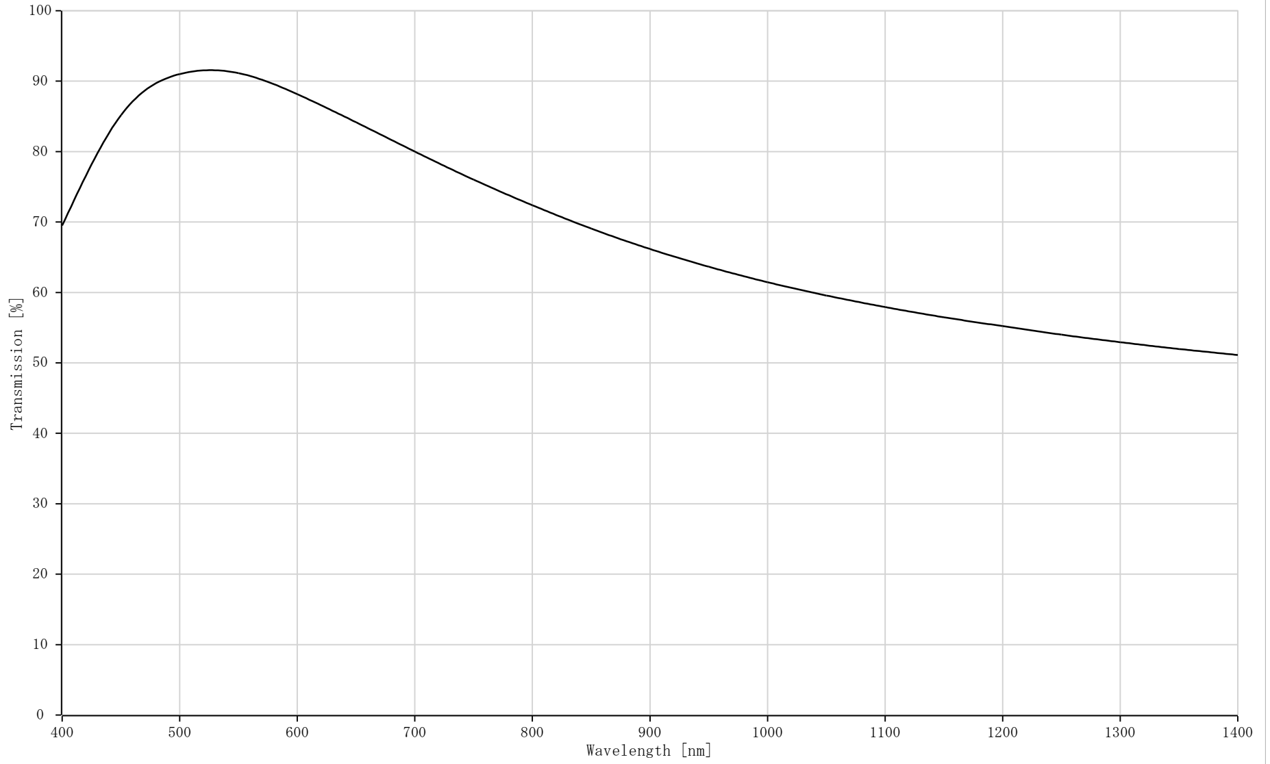
LM12JC5MC-WP Transmission
