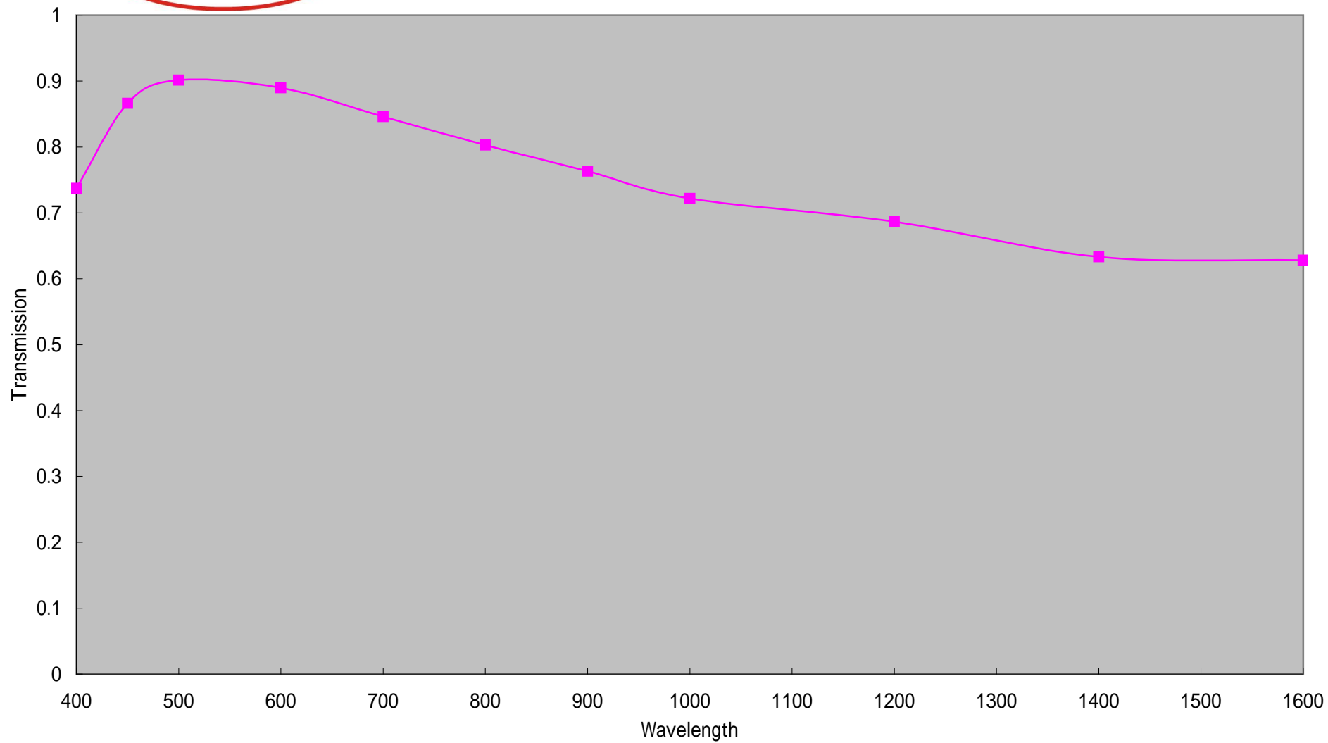
LM100JC (948) Transmission
