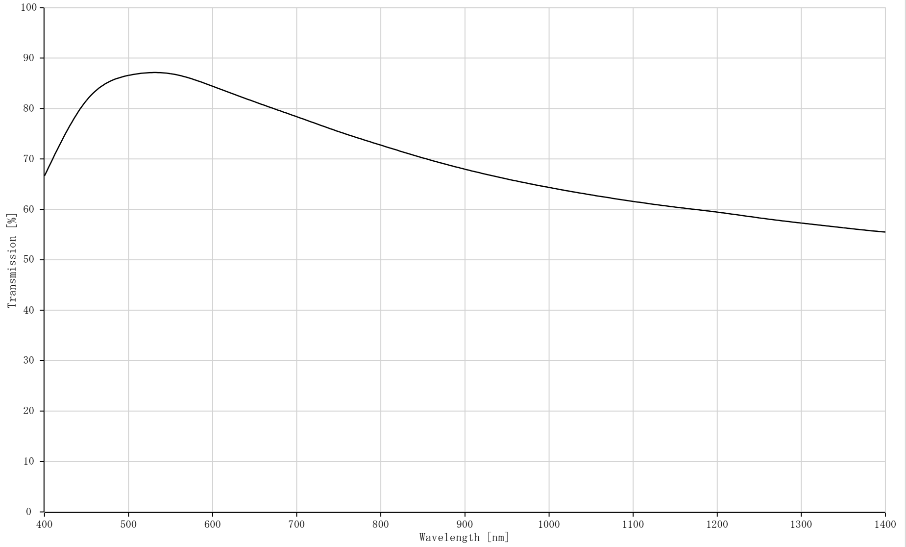
LM25EC-IR Transmission
