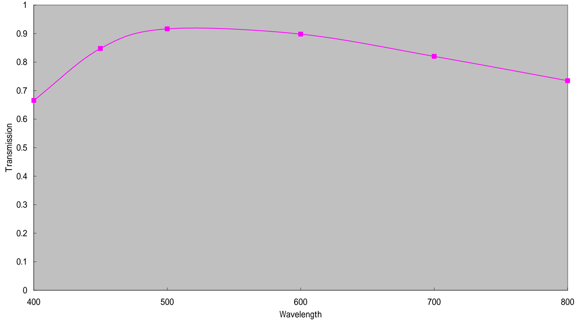
LM12JC (638) Transmission
